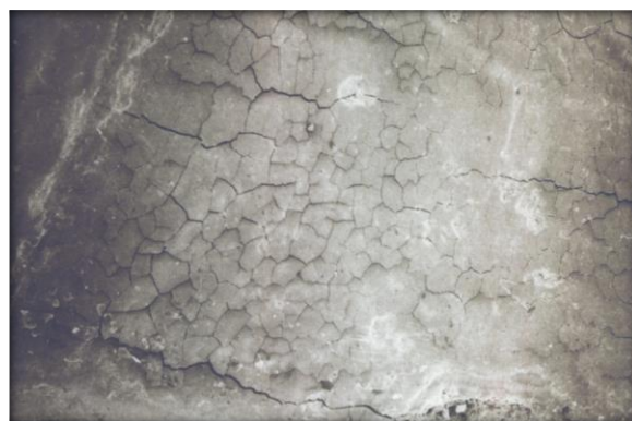
Fig. 8: SEM view of test side instrumented for 50 strokes with curette. 50x
